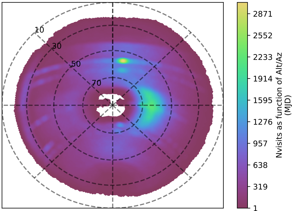
weather_cloudso14v3.4_10yrs r band: Nvisits as function of Alt/Az
