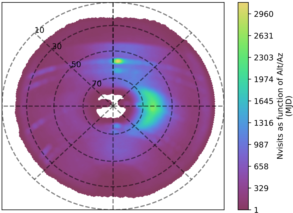
weather_cloudso14v3.4_10yrs i band: Nvisits as function of Alt/Az
