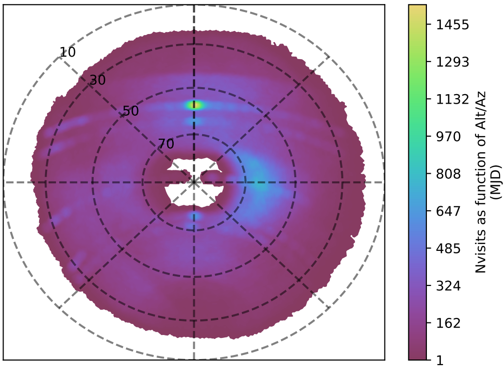
weather_cloudso14v3.4_10yrs g band: Nvisits as function of Alt/Az
