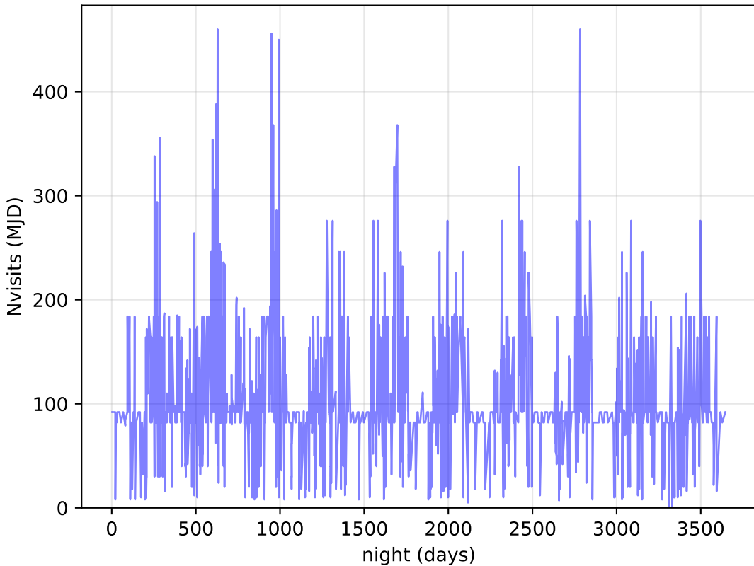
weather_cloudso14v3.4_10yrs DDF: Nvisits
