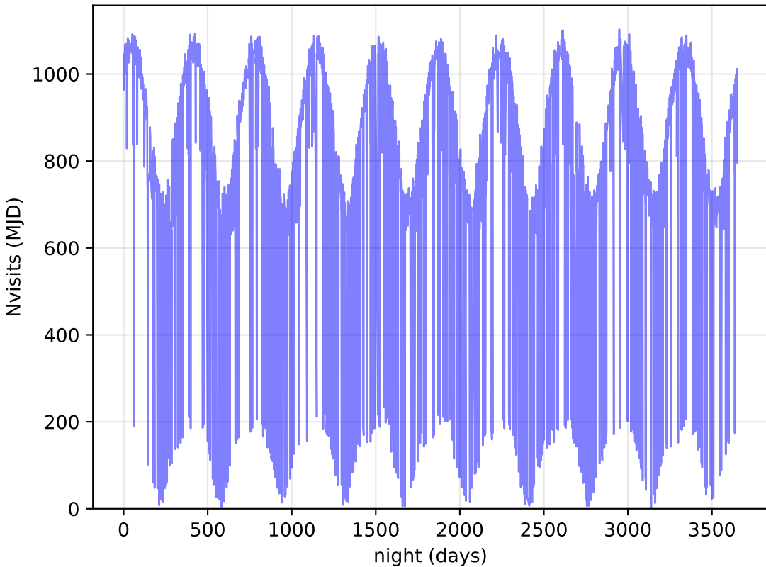
weather_cloudso14v3.4_10yrs All visits: Nvisits
