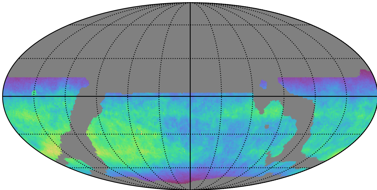
weather_cloudso14v3.4_10yrs WFD z band: Normalized Teff
