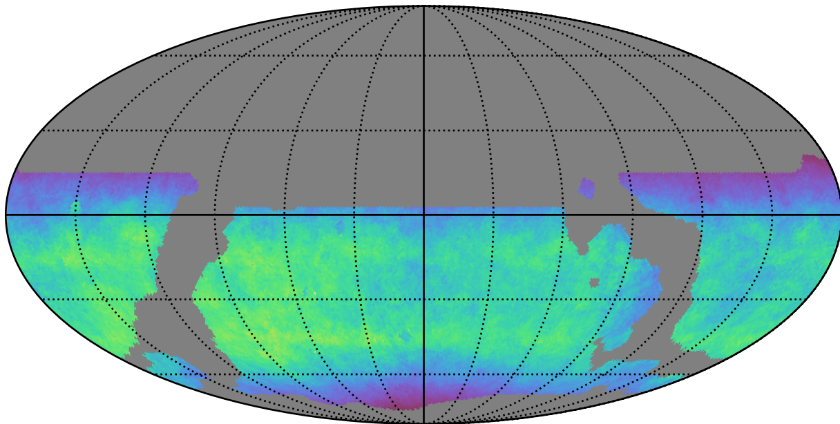
weather_cloudso14v3.4_10yrs WFD y band: Normalized Teff
