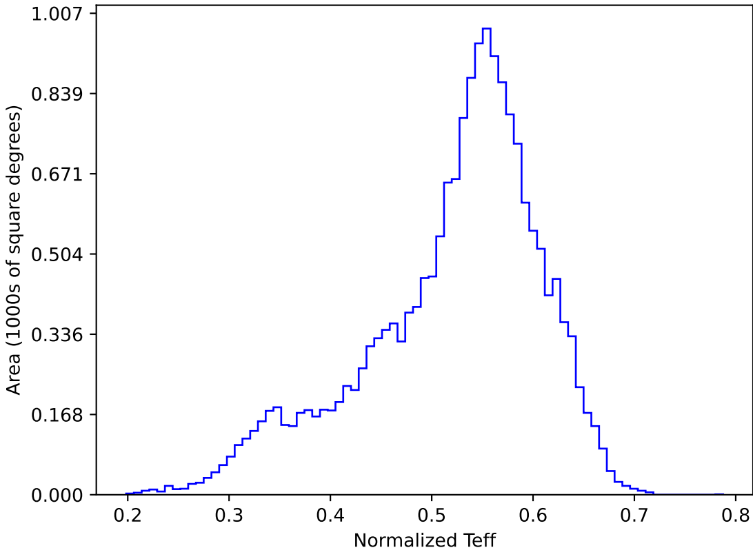
weather_cloudso14v3.4_10yrs WFD y band: Normalized Teff
