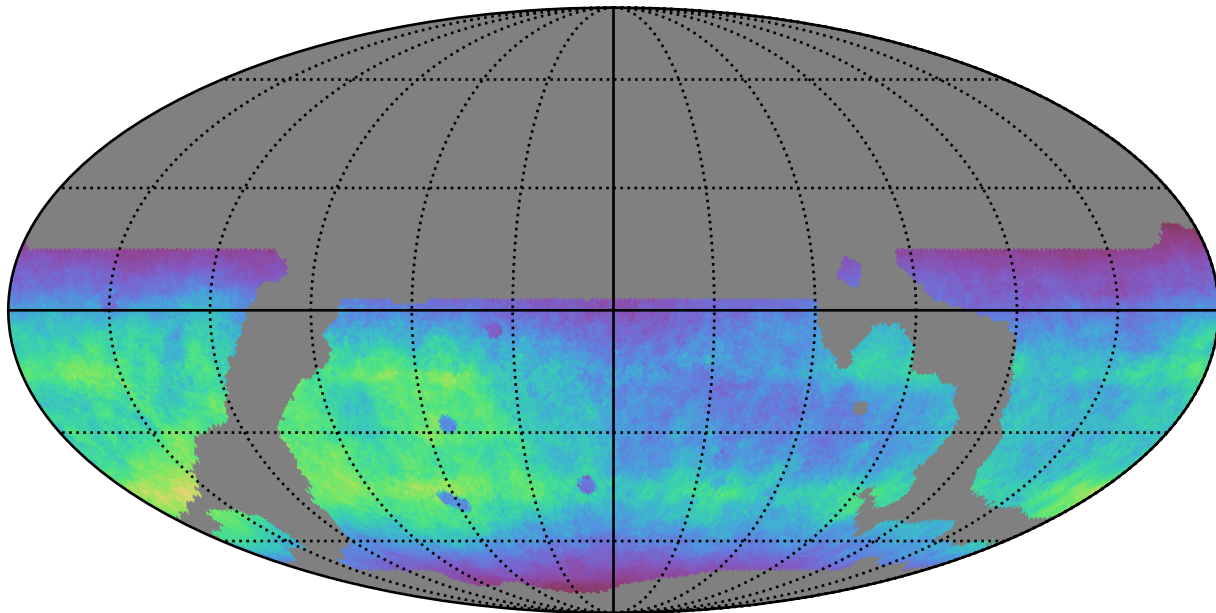
weather_cloudso14v3.4_10yrs WFD r band: Normalized Teff
