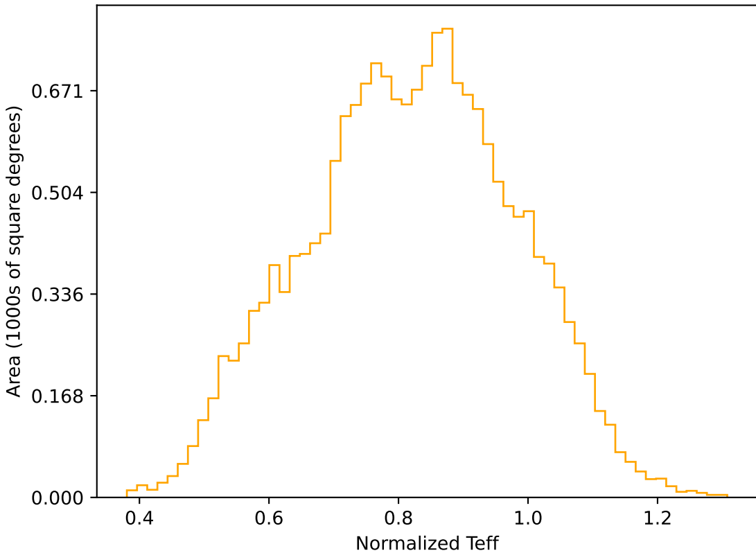
weather_cloudso14v3.4_10yrs WFD r band: Normalized Teff
