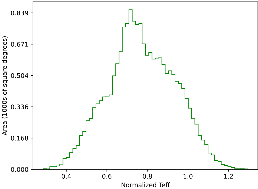
weather_cloudso14v3.4_10yrs WFD g band: Normalized Teff
