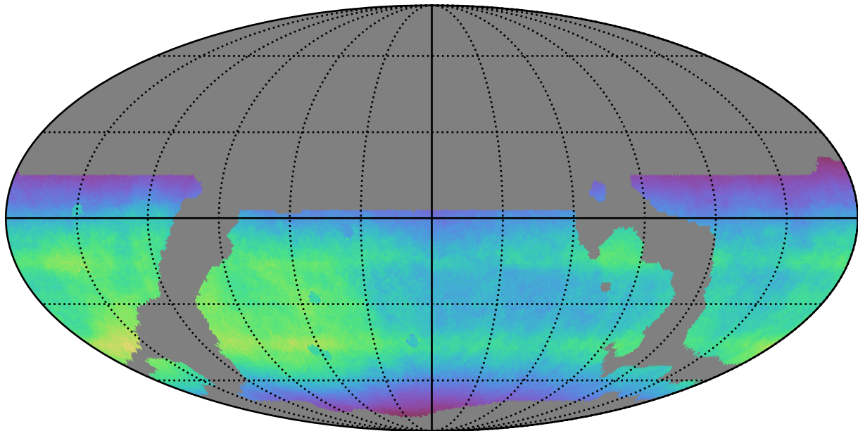
weather_cloudso14v3.4_10yrs WFD all bands: Normalized Teff
