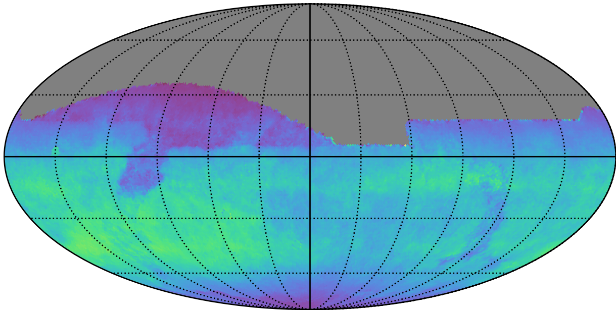
weather_cloudso14v3.4_10yrs All sky z band: Normalized Teff
