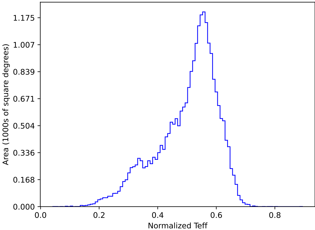
weather_cloudso14v3.4_10yrs All sky y band: Normalized Teff
