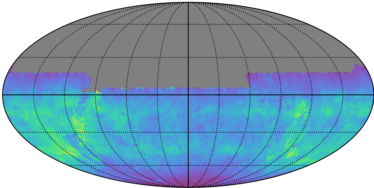
weather_cloudso14v3.4_10yrs All sky u band: Normalized Teff
