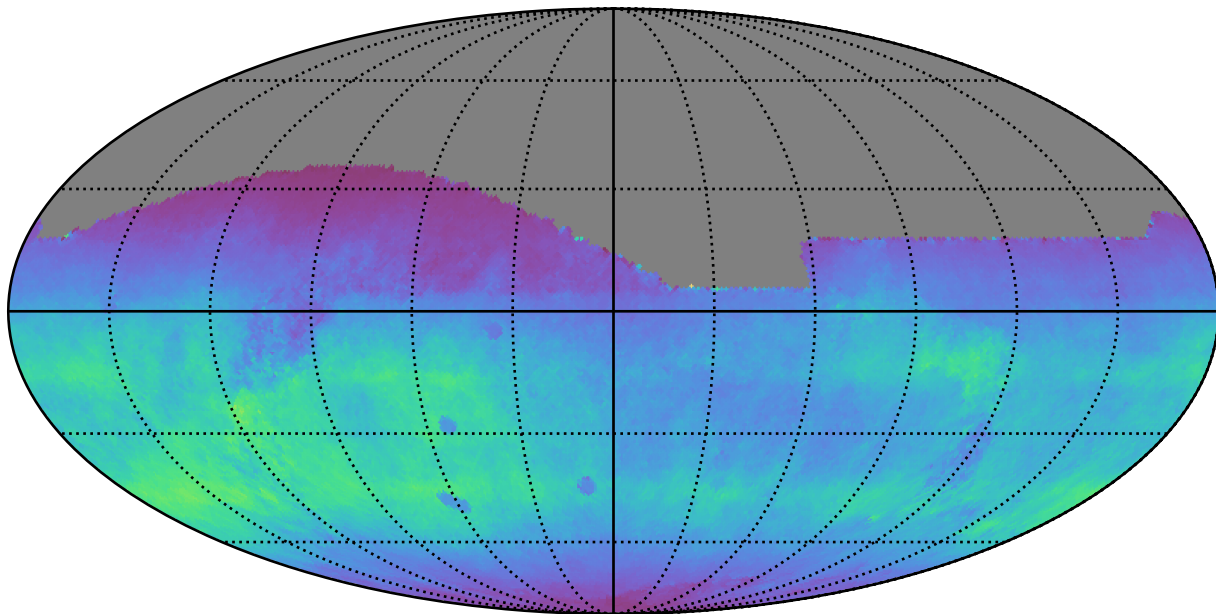
weather_cloudso14v3.4_10yrs All sky r band: Normalized Teff
