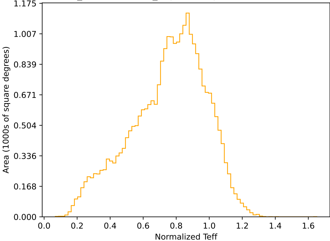
weather_cloudso14v3.4_10yrs All sky r band: Normalized Teff
