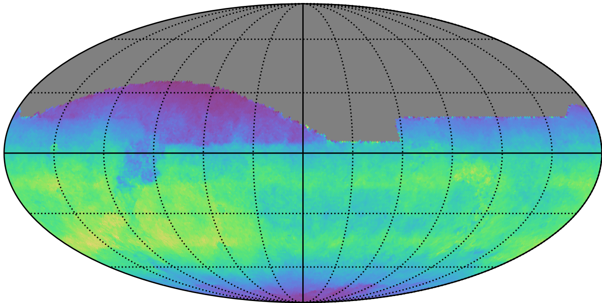
weather_cloudso14v3.4_10yrs All sky i band: Normalized Teff
