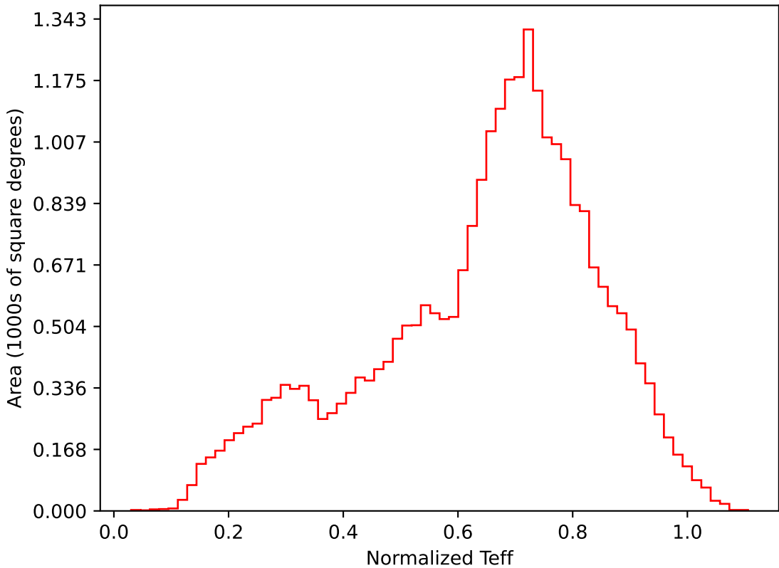
weather_cloudso14v3.4_10yrs All sky i band: Normalized Teff
