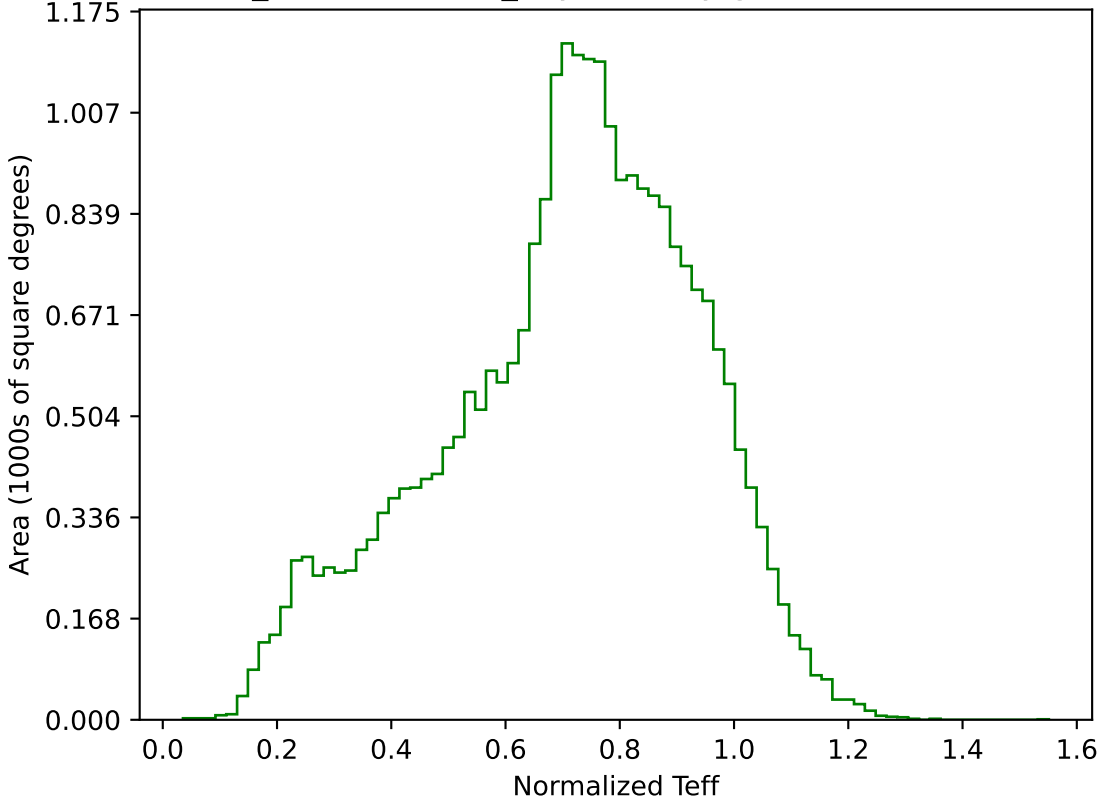
weather_cloudso14v3.4_10yrs All sky g band: Normalized Teff
