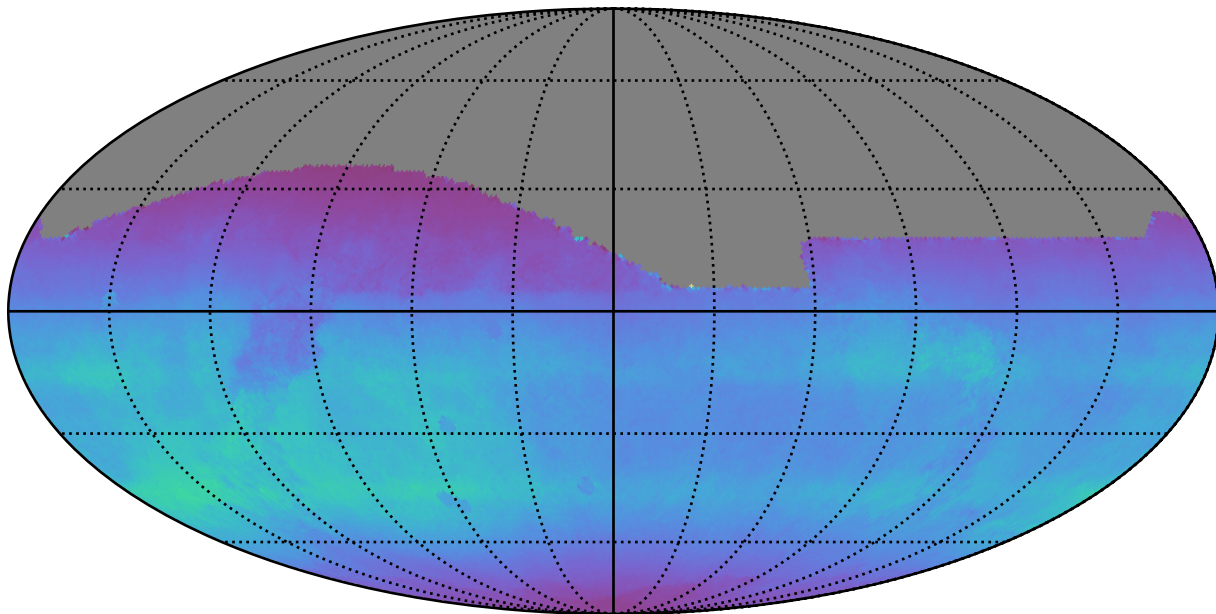
weather_cloudso14v3.4_10yrs All sky all bands: Normalized Teff
