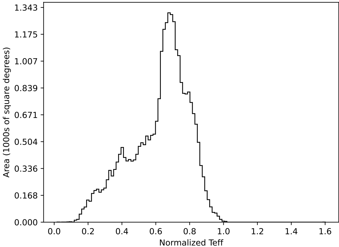
weather_cloudso14v3.4_10yrs All sky all bands: Normalized Teff
