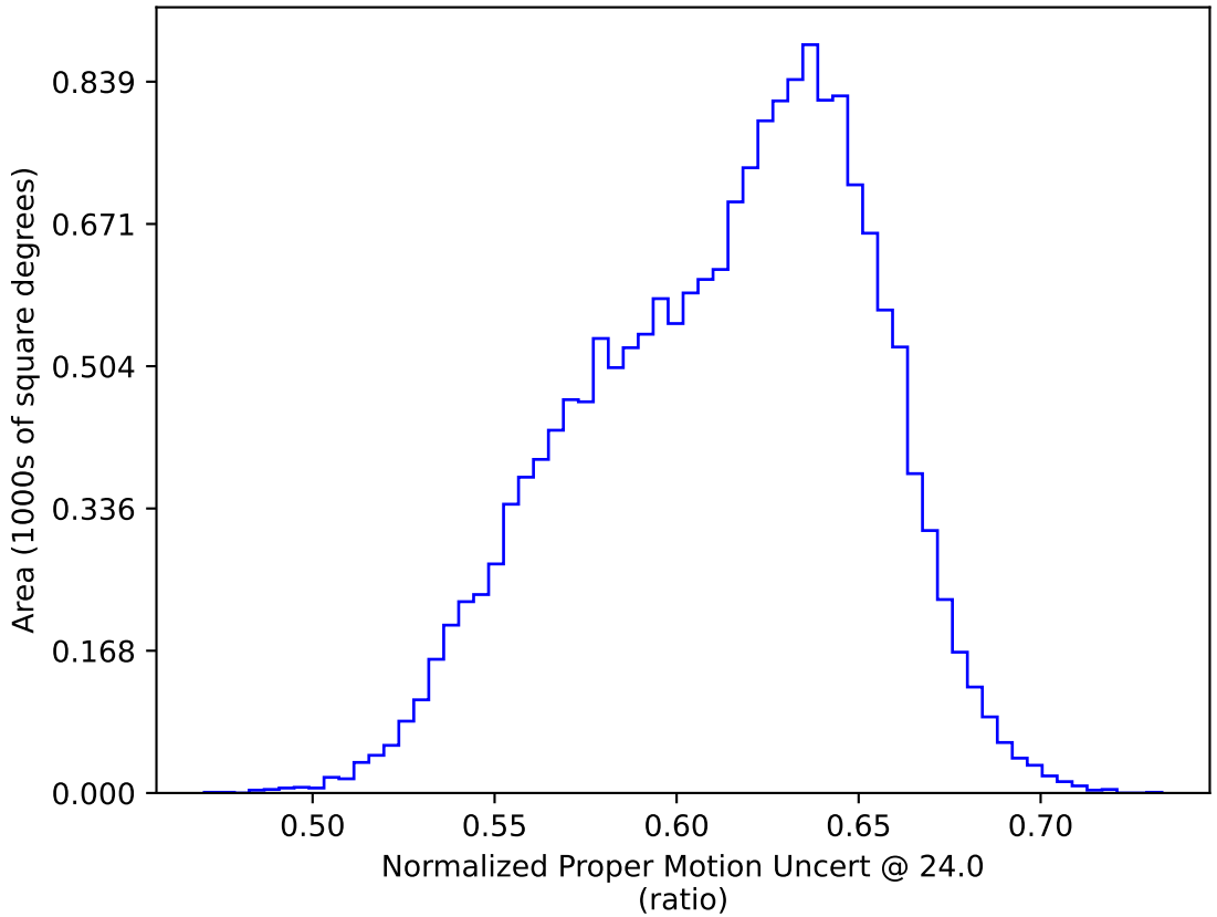
weather_cloudso14v3.4_10yrs WFD: Normalized Proper Motion Uncert @ 24.0
