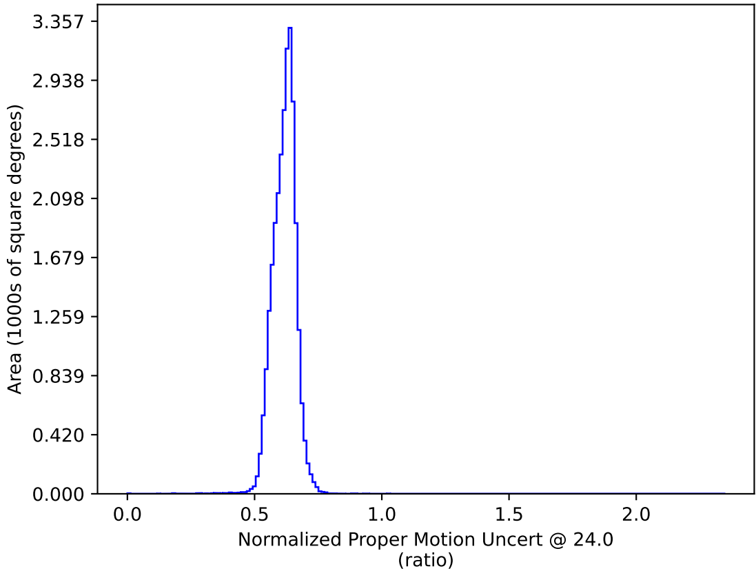
weather_cloudso14v3.4_10yrs All sky: Normalized Proper Motion Uncert @ 24.0
