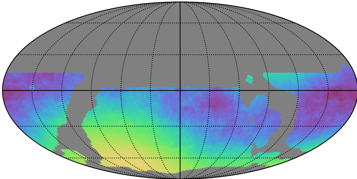
weather_cloudso14v3.4_10yrs WFD: Normalized Parallax Uncert @ 24.0
