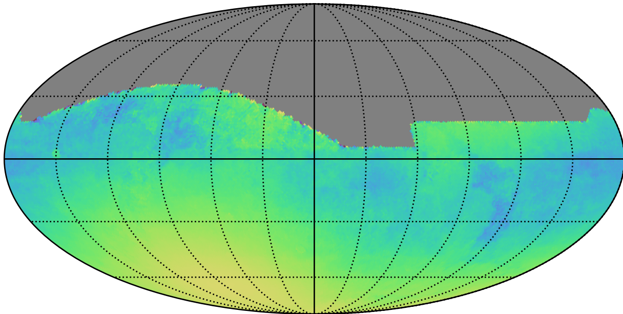
weather_cloudso14v3.4_10yrs All sky: Normalized Parallax Uncert @ 24.0
