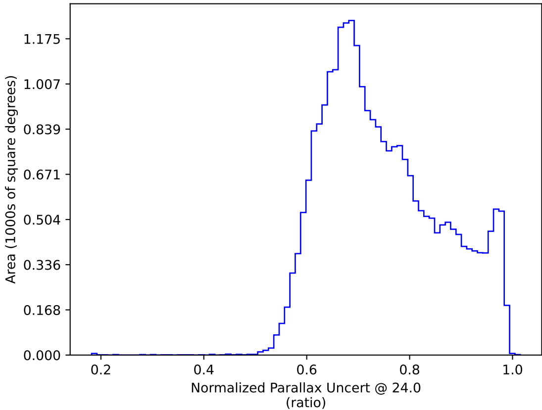
weather_cloudso14v3.4_10yrs All sky: Normalized Parallax Uncert @ 24.0
