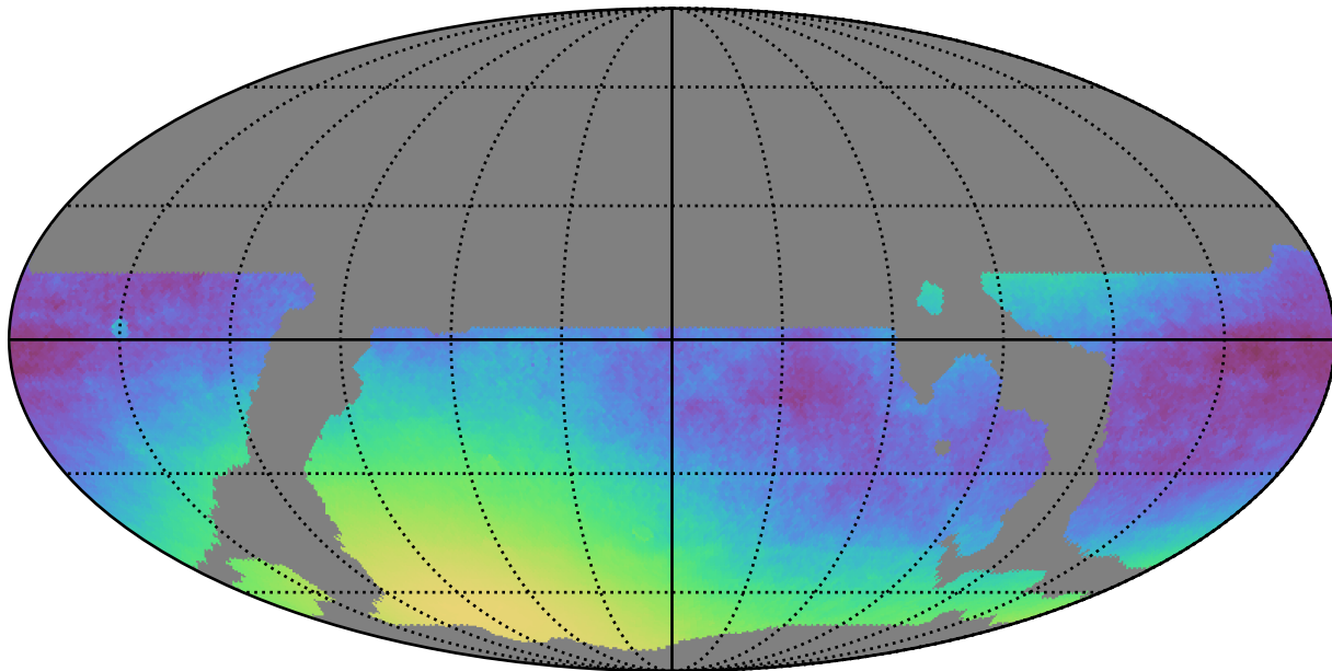
weather_cloudso14v3.4_10yrs WFD: Normalized Parallax Uncert @ 22.4
