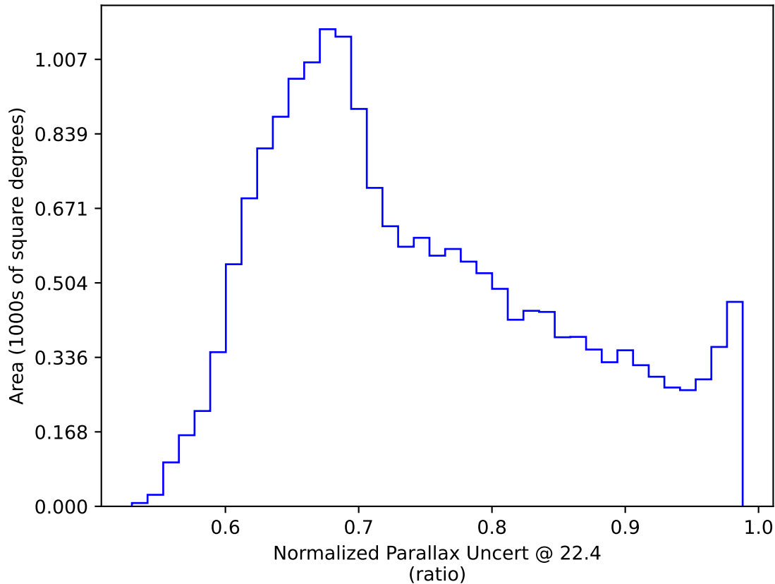
weather_cloudso14v3.4_10yrs WFD: Normalized Parallax Uncert @ 22.4
