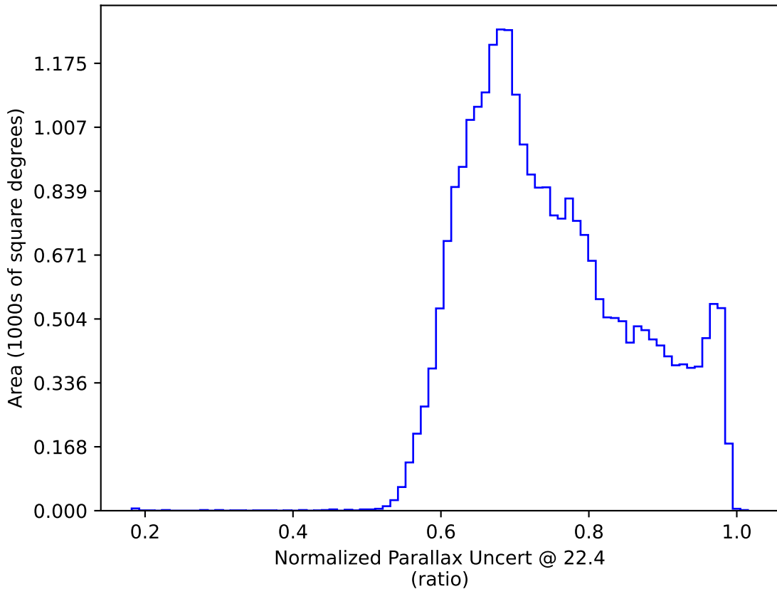
weather_cloudso14v3.4_10yrs All sky: Normalized Parallax Uncert @ 22.4
