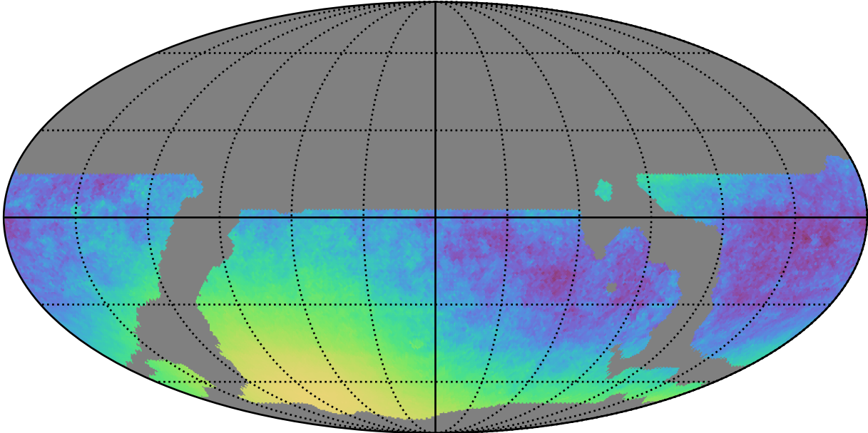
weather_cloudso14v3.4_10yrs WFD y band only: Normalized Parallax Uncert @ 21.3
