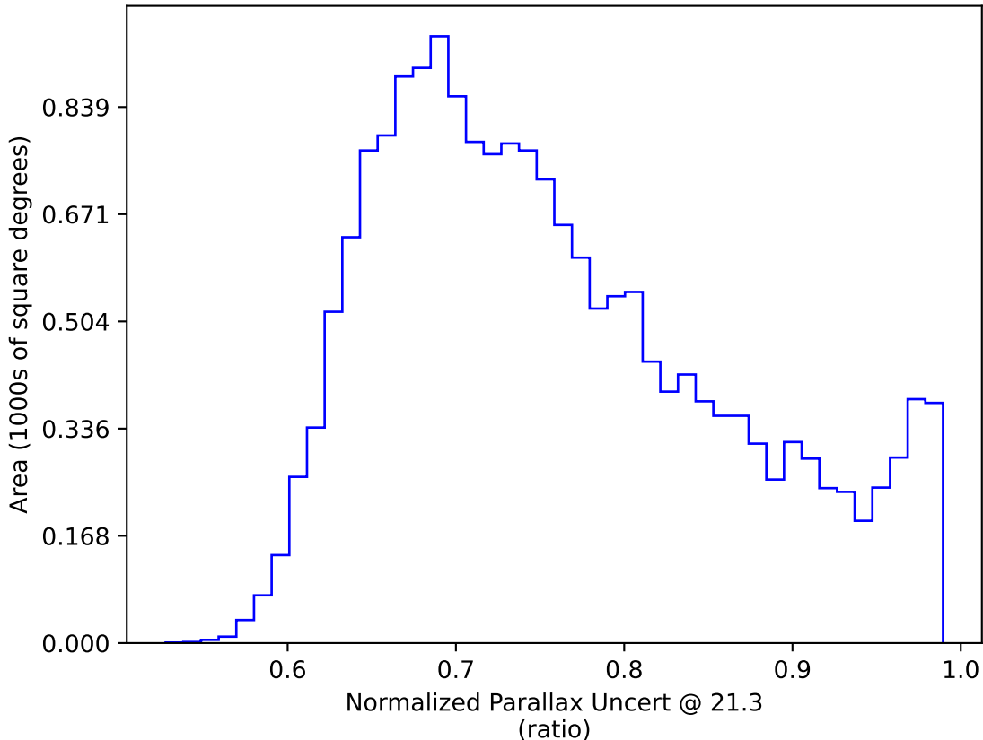
weather_cloudso14v3.4_10yrs WFD y band only: Normalized Parallax Uncert @ 21.3
