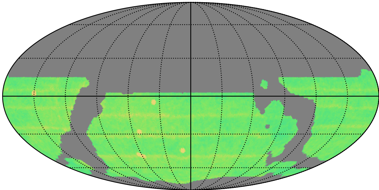
weather_cloudso14v3.4_10yrs WFD all bands: N Unique Nights
