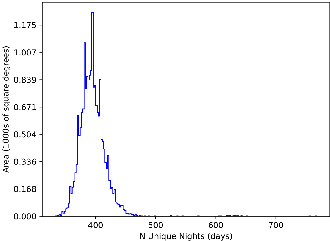
weather_cloudso14v3.4_10yrs WFD all bands: N Unique Nights
