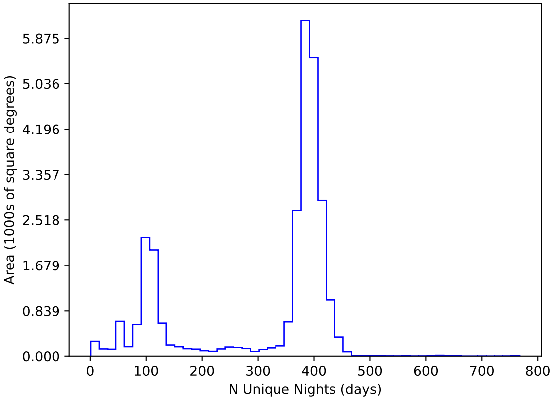
weather_cloudso14v3.4_10yrs All sky all bands: N Unique Nights
