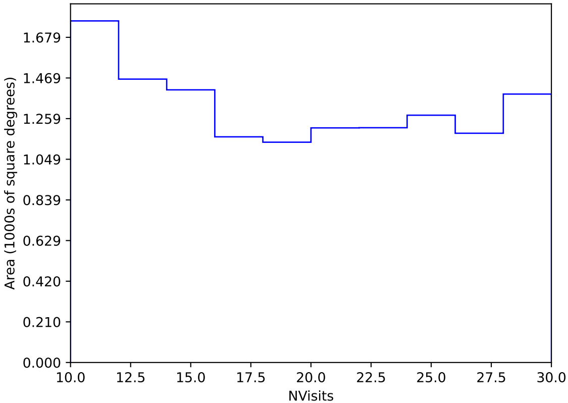
weather_cloudso14v3.4_10yrs Yr 3-4 y band: NVisits
