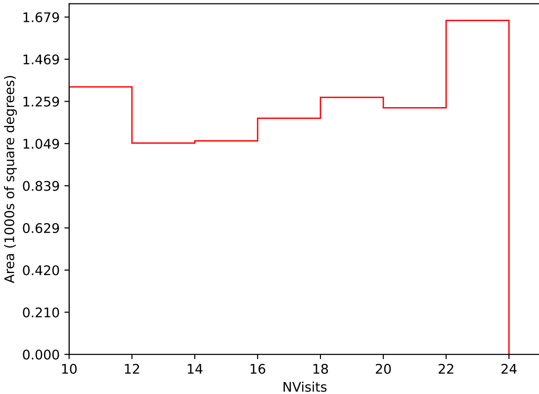
weather_cloudso14v3.4_10yrs Yr 3-4 i band: NVisits
