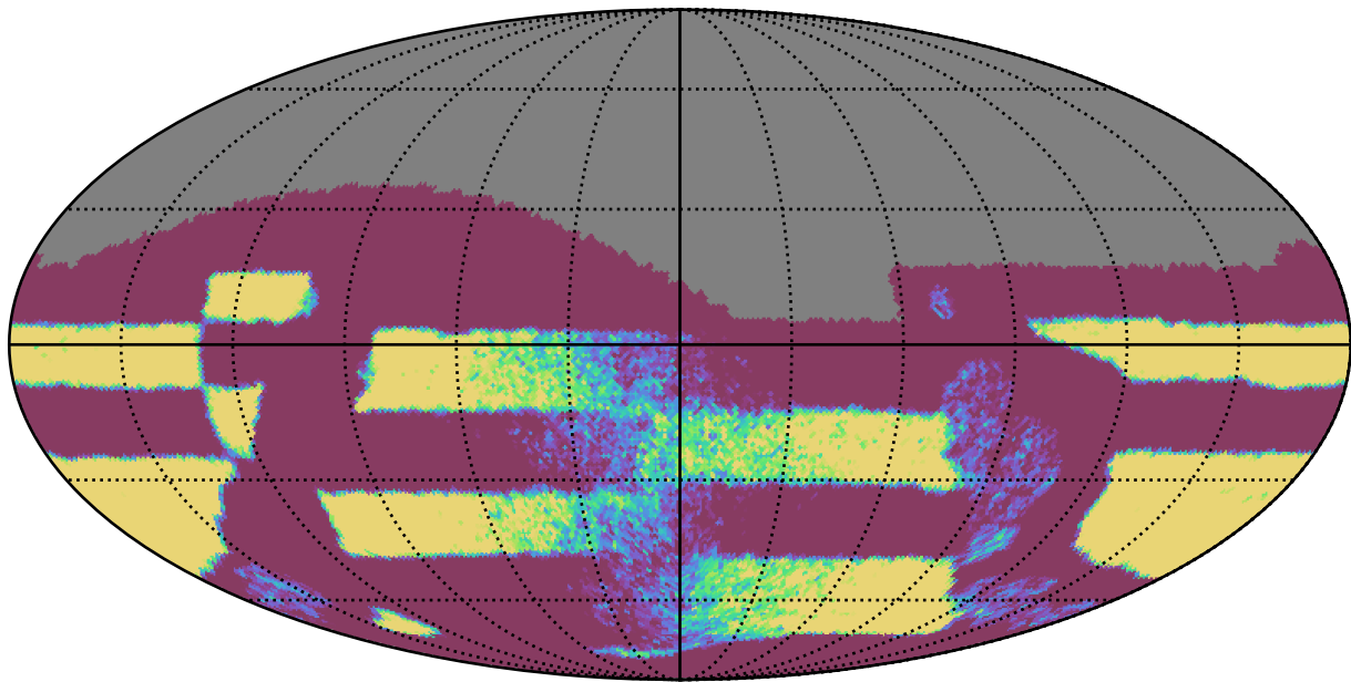
weather_cloudso14v3.4_10yrs Yr 3-4 all bands: NVisits
