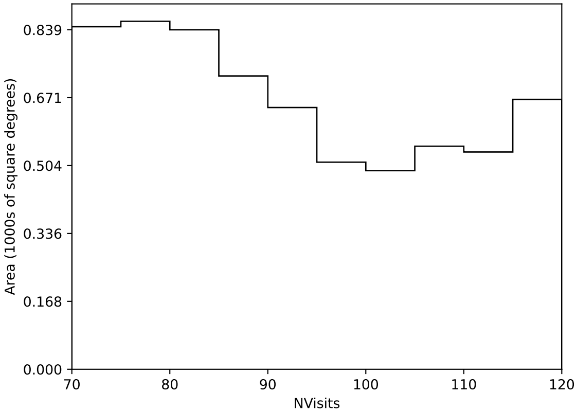
weather_cloudso14v3.4_10yrs Yr 3-4 all bands: NVisits
