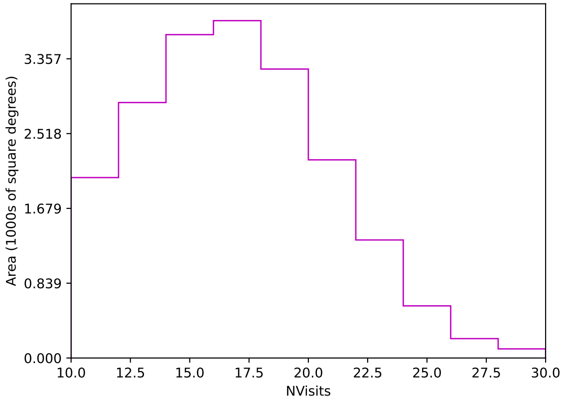
weather_cloudso14v3.4_10yrs Yr 1 z band: NVisits
