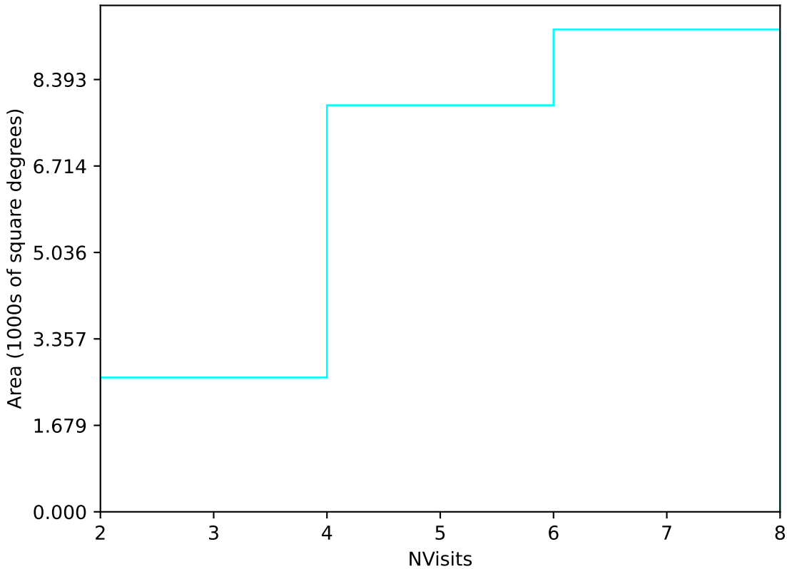
weather_cloudso14v3.4_10yrs Yr 1 u band: NVisits
