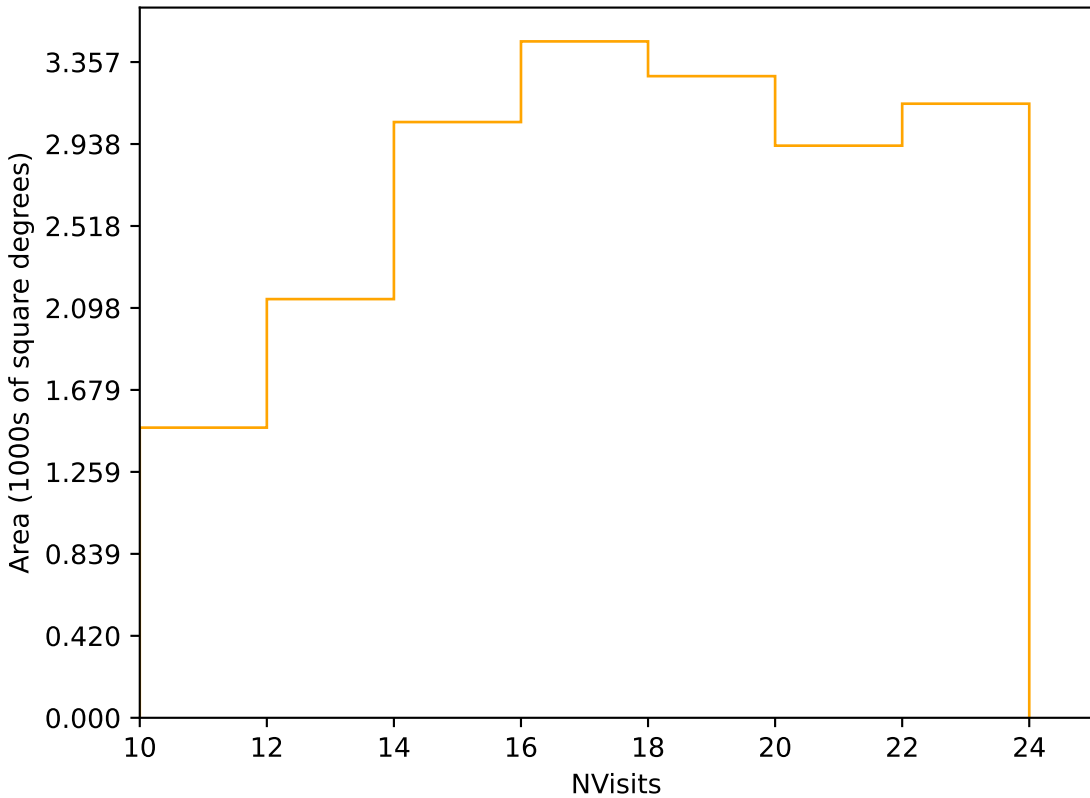
weather_cloudso14v3.4_10yrs Yr 1 r band: NVisits
