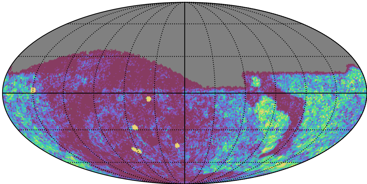
weather_cloudso14v3.4_10yrs Yr 1 g band: NVisits
