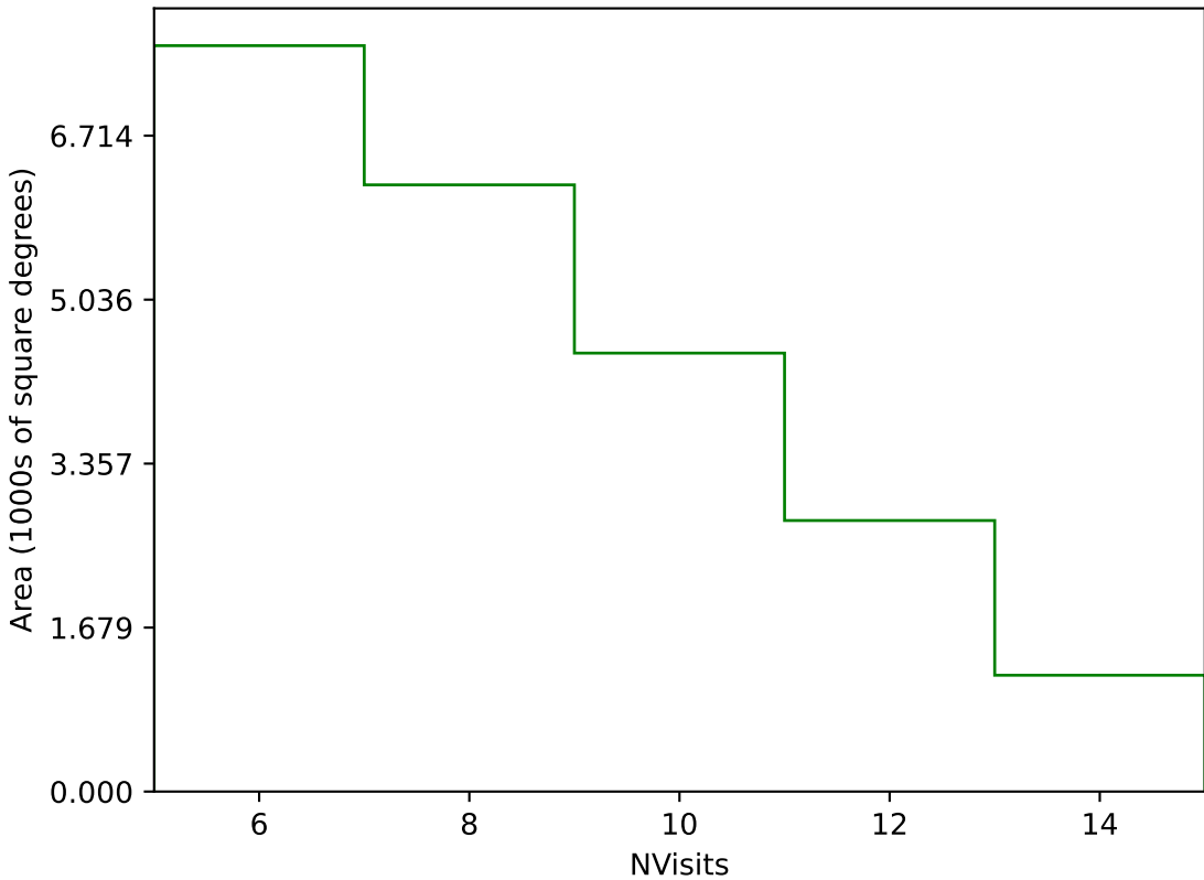
weather_cloudso14v3.4_10yrs Yr 1 g band: NVisits
