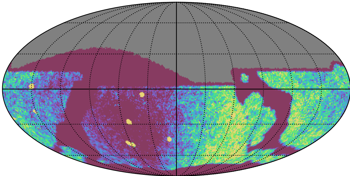
weather_cloudso14v3.4_10yrs Yr 1 all bands: NVisits
