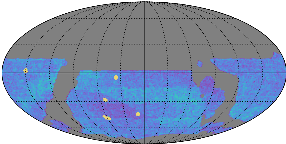
weather_cloudso14v3.4_10yrs WFD all bands: NVisits
