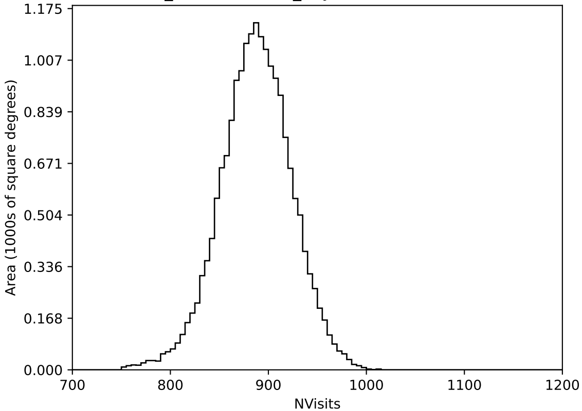
weather_cloudso14v3.4_10yrs WFD all bands: NVisits
