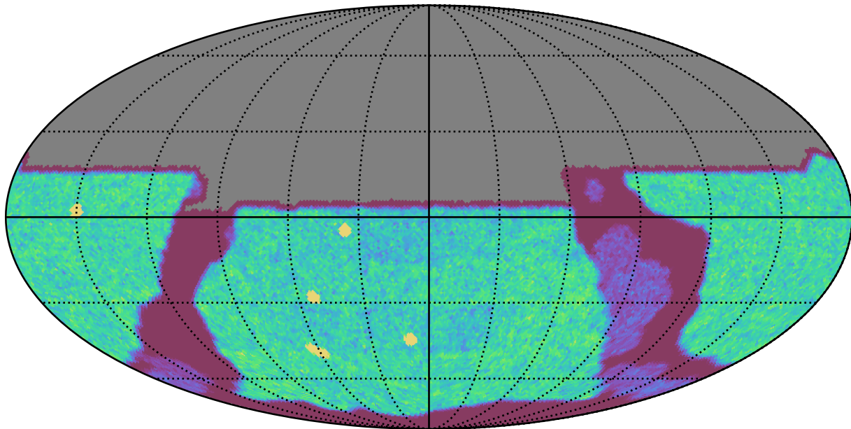
weather_cloudso14v3.4_10yrs All sky u band: NVisits
