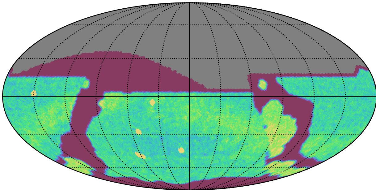
weather_cloudso14v3.4_10yrs All sky r band: NVisits
