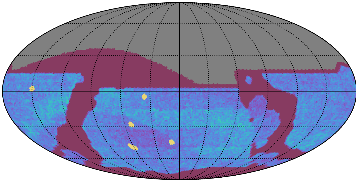
weather_cloudso14v3.4_10yrs All sky all bands: NVisits
